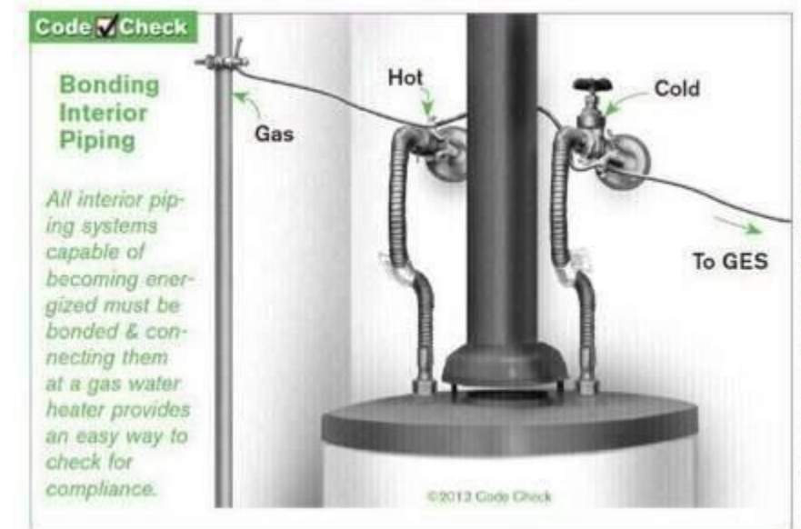
ADD ELECTRICAL BONDING TO INTERIOR PIPING
