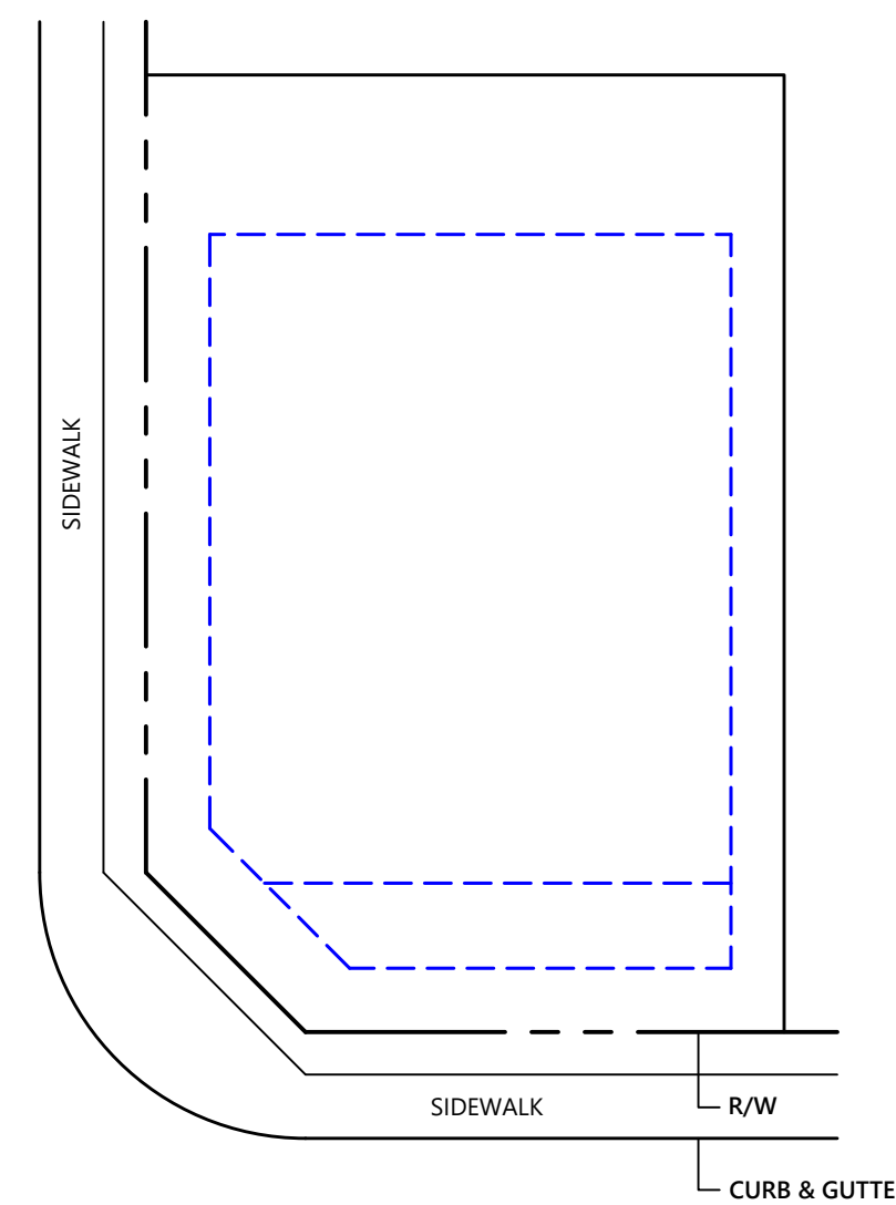
TYPICAL CORNER LOT SETBACKS SCALE: 1" = 20'
