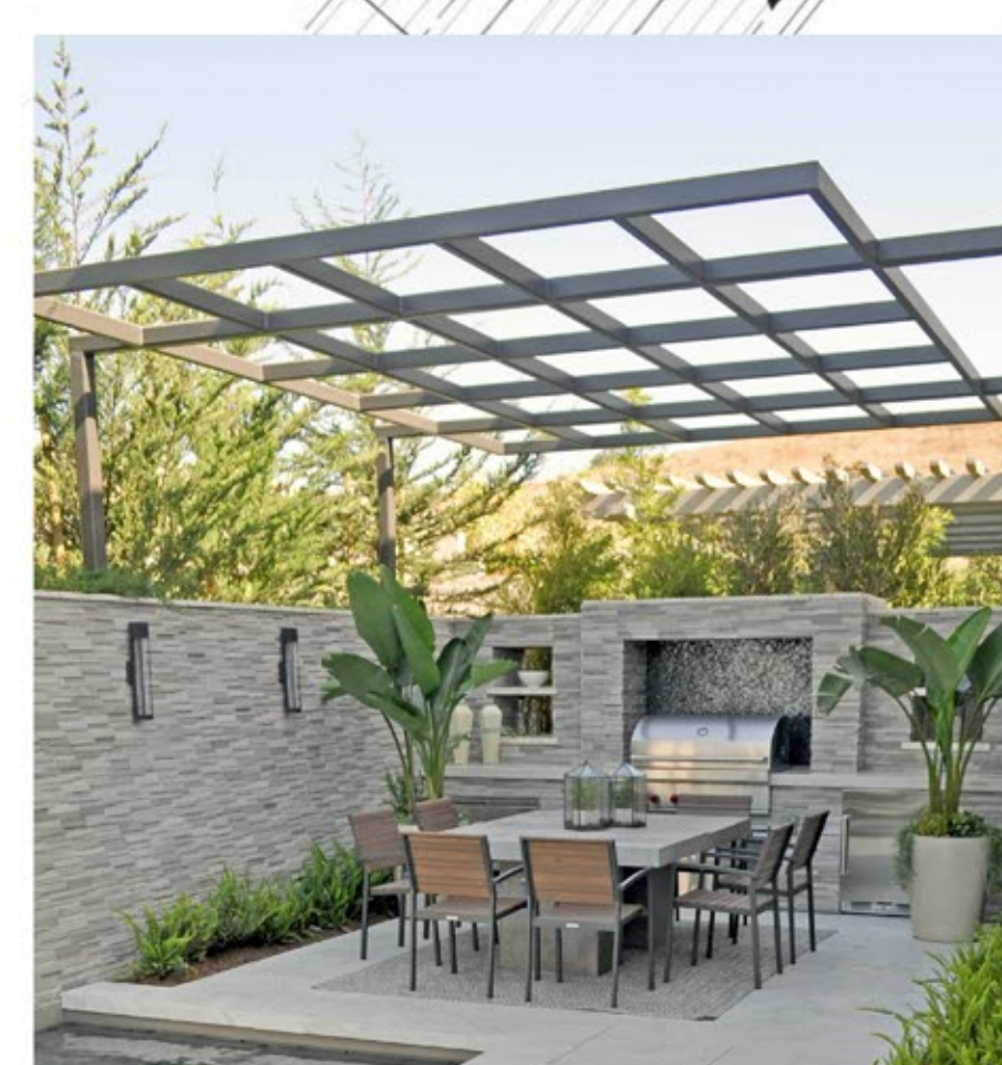
FREESTANDING ALUMINUM SPACE FRAME ON STONE COLUMNS TO MATCH ARCHITECTURE
