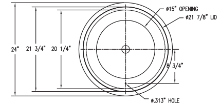
1 TOP VIEW OF TF1840 WASTE CONTAINER SHOWN WITHOUT LID Scale: 1/8" = 1"
